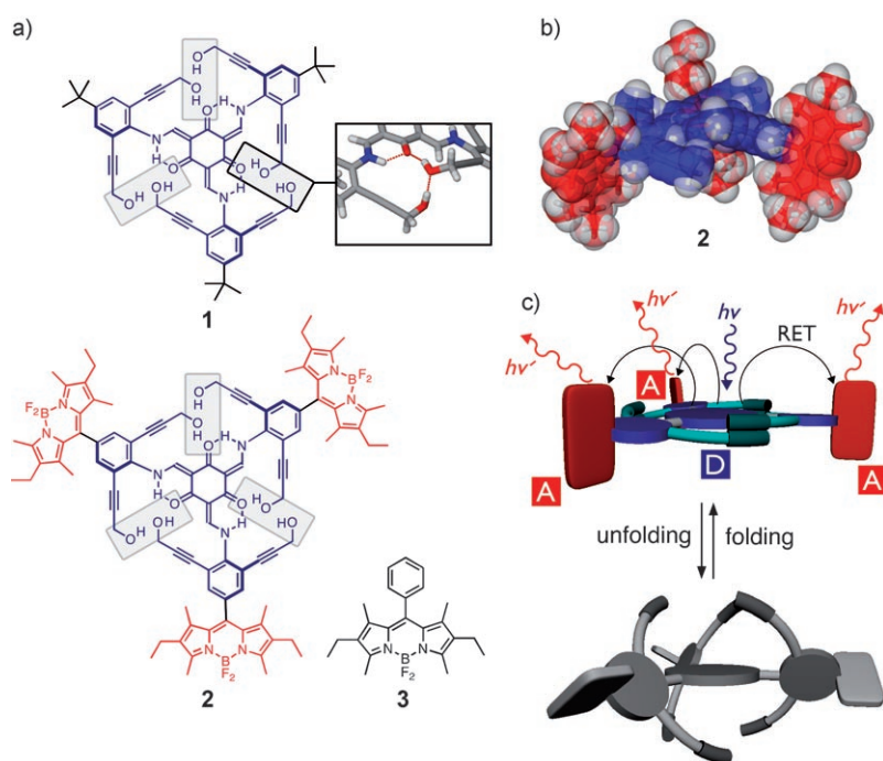
Figure 2. a) Chemical structures of compounds 1–3 with a close-up view of the \text{O}_{\text{hydroxy}}\cdots\text{H}\cdots\text{O}_{\text{carbonyl}} hydrogen-bonding network (shown as capped-stick model). [11a,b] b) Energy-minimized (PM3) structure of compound 2 in which the tris( N -salicylideneaniline) and BODIPY units are color-coded with blue and red, respectively. c) Schematic representation of conformational switching between the emissive “folded” (top) and the nonemissive “unfolded” (bottom) states of compound 2 (D = energy donor; A = energy acceptor).
