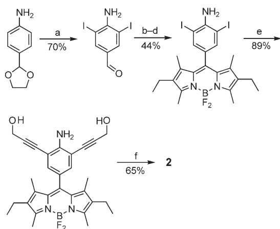
Scheme 1. Synthetic route to compound 2. [15] a) \text{Ag}_2\text{SO}_4 , \text{I}_2 , EtOH, room temperature (RT); b) 3-ethyl-2,4-dimethylpyrrole (2.1 equiv), \text{CH}_2\text{Cl}_2 , RT; c) 2,3-dichloro-5,6-dicyano-1,4-benzoquinone (DDQ) (1.1 equiv), \text{CH}_2\text{Cl}_2 , RT; d) \text{Et}_3\text{N} (10 equiv), \text{BF}_3\cdot\text{Et}_2\text{O} (15 equiv), \text{CH}_2\text{Cl}_2 , \Delta ; e) \text{HCCHCH}_2\text{OH} , [\text{PdCl}_2(\text{PPh}_3)_2] (2 mol%), \text{CuI} (3 mol%), i\text{Pr}_2\text{NH}/\text{THF} , RT; f) 1,3,5-triformylphloroglucinol, EtOH, \Delta .
